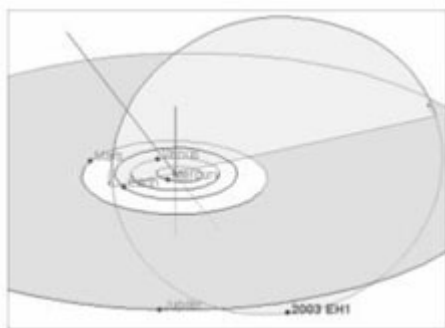
Orbit and position of 2003 EH1 on January 4, 2003.
