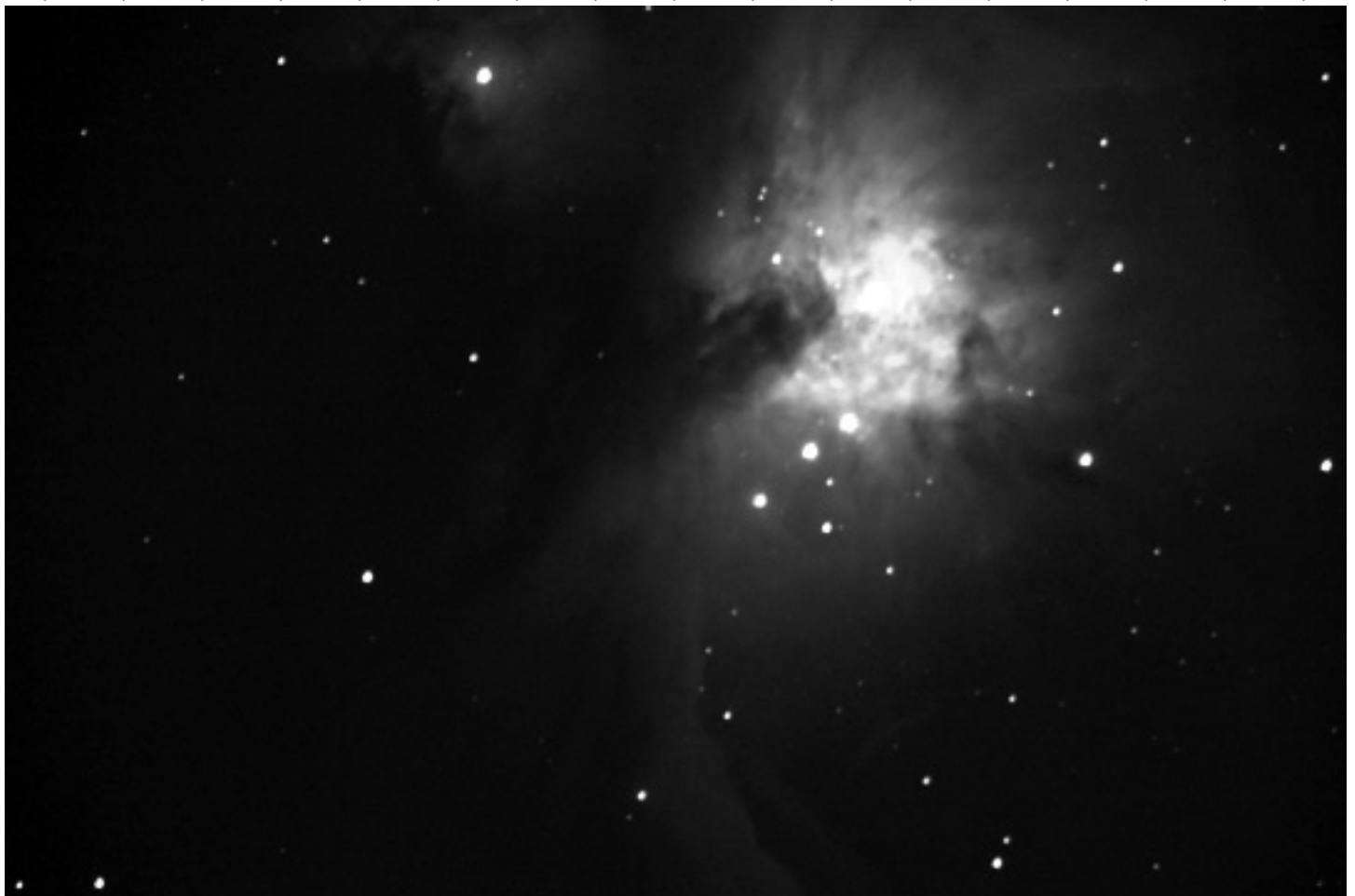
This image of the Orion Nebula (M42) was taken during the early morning of October 30, 2011. The imager was a Canon Rebel EOS T2i. The telescope is a Meade LX 200 ACF 12". This image is a single 30 second exposure with ISO setting of 3200. It was minimally processed in Photoshop CS2 using a product called "Annie's Actions" sold by Anna Morris. Image by Paul Kohlmeier
